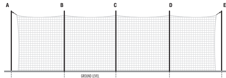
Ropes attach to the hanging-loop assemblies on crossbars A, B, C, D, and E.
