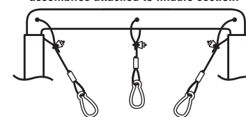
Figure 2 Close-up view of the hanging-loop assemblies attached to middle section.
